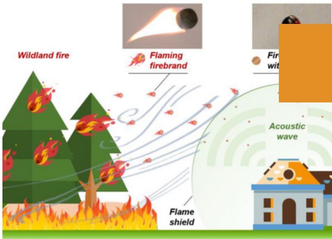
Extinction of flaming firebrand at wildland-urban interface
